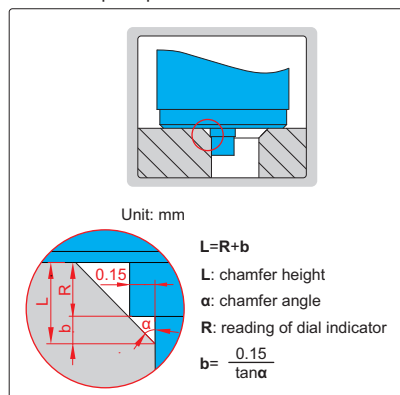
principle of measurement
