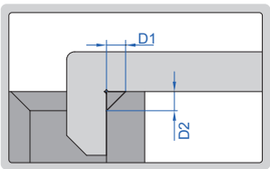
internal chamfer
