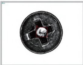
cross recess excess material
