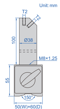
MAGNETIC BASE (mm)
