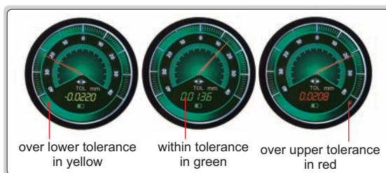
■ Meet DIN863-3 ■ Absolute encoder, the original data remains after power off ■ Measuring stroke of anvil: >1mm ■ Reading in digital and analog ■ Button function: on/off, zero setting, mm/inch, tolerance, display setting, bluetooth, signal mode setting, data output ■ Android and iPhone APP, USB type-C cable are included ■ Carbide measuring faces ■ Power: rechargeable Li-battery, for 20 hours continuous working (bluetooth transmission reduces working hours) ■ Optional accessory: gauge blocks grade 0 ■ (4101-A series) , for zero setting
