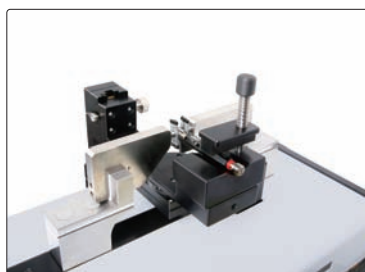
measuring thread plug gauges (manual mode)
