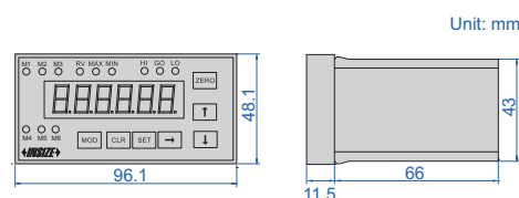
connected with 7107-11 , 7107-12 , 7107-11V or 7107-12V linear gauge
