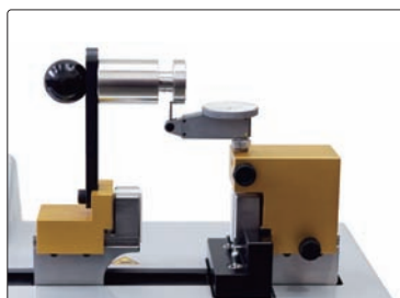
dial test indicator calibration
